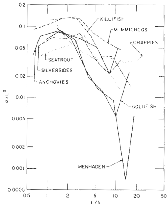
FIGURE 7.—Average measured dorsal-aspect acoustic cross-sections for different species of fish. (From Love, 1971.)
