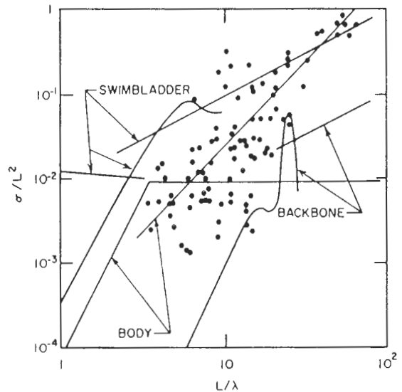
FIGURE 3.—Side-aspect acoustic cross-sections determined by Haslett.
