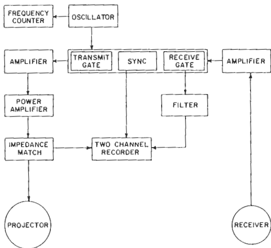
FIGURE 1.—Typical target strength measurement system electronics.
